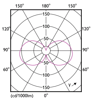
Light Distribution Diagram - MAS LEDBulbND2.3-40W E27840 A60CL G EELA
