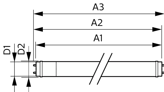
CorePro LEDtube 1500mm HO 24W 840 T8
