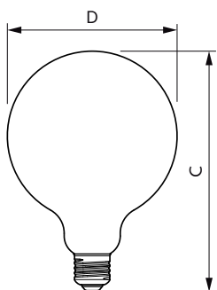
G120 220-240V 75W 1055lm 2700K E27 ND FR
