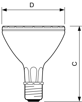
MASTERCcolour CDM-R Elite 70W/930 E27 PAR30L 40D
