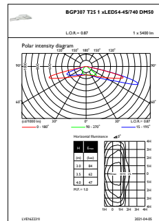
OFPL1_BGP307T251xLED54-4S740DM50
