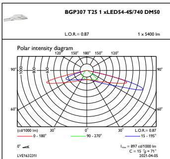
OFPC1_BGP307T251xLED54-4S740DM50
