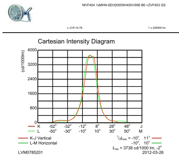
OFCC_MVF404 1xMHN-SEH2000W/400V/956 B6 +ZVF403 GS-Cartesian Outdoor (combined)
